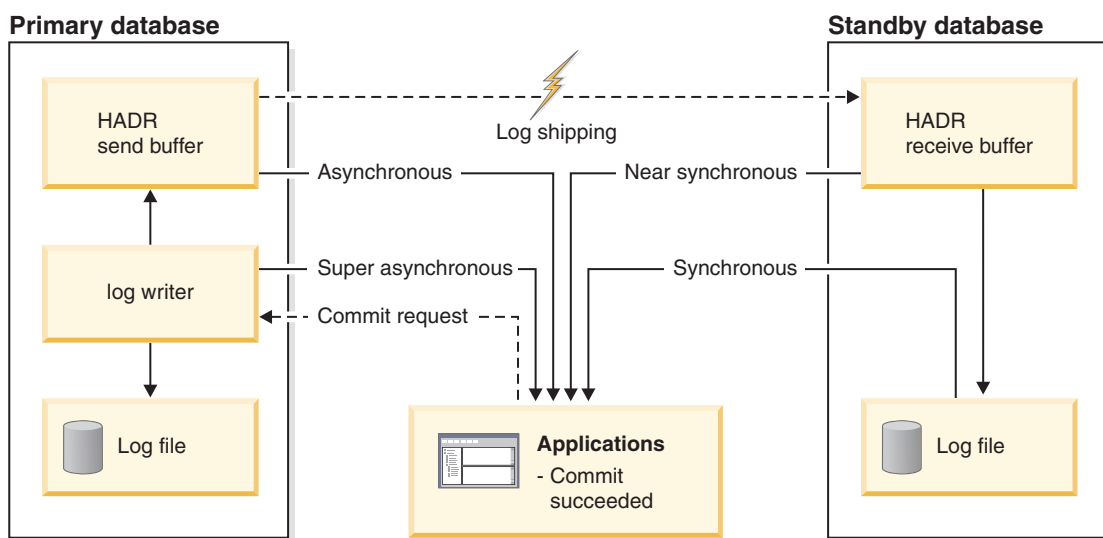
Figure 52. Synchronization modes for high availability and disaster recovery (HADR)
