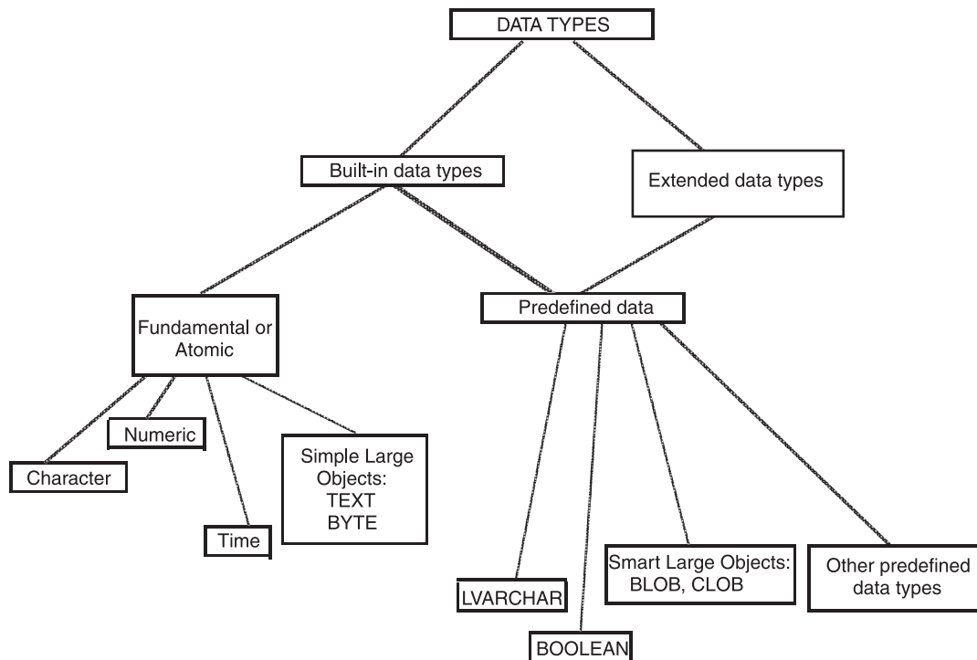
Figure 8-1. IBM Informix data types
