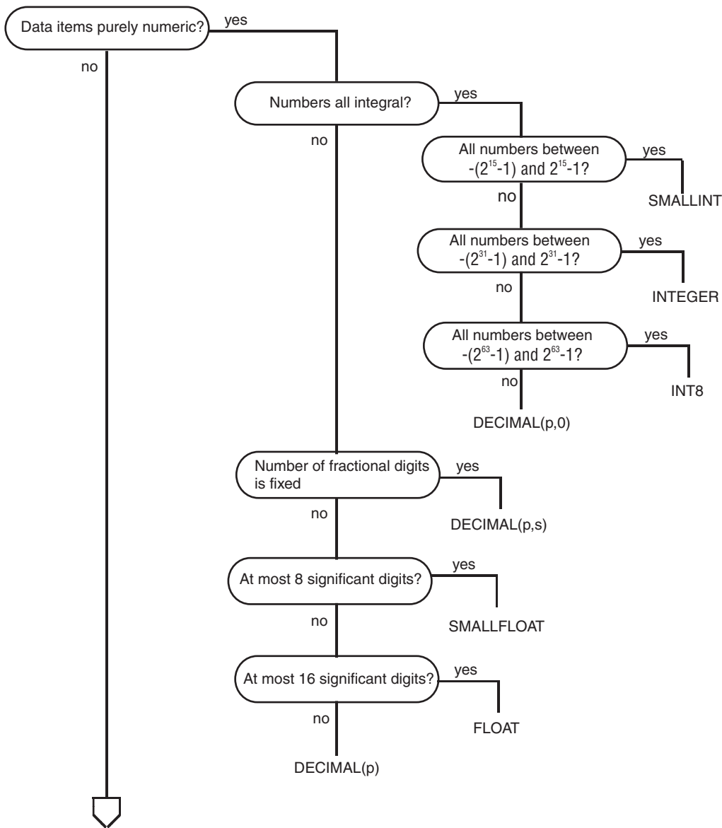
Figure 3-1. Select a data type
