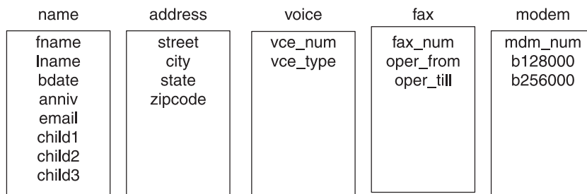
Figure 2-11. Attributes for the telephone directory example
