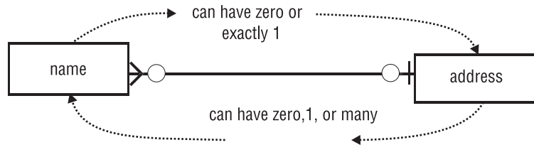
Figure 2-14. Reading an entity-relationship diagram
