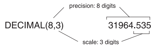
Figure 3-3. The relation between precision and scale in a fixed-point number
