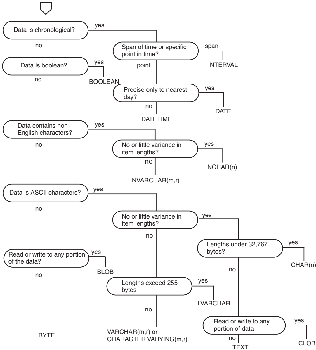
Figure 3-2. Select a data type (continued)
