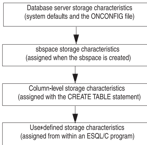
Figure 8-1. Inheritance hierarchy for storage characteristics
