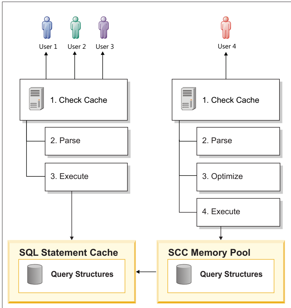
Figure 4-3. Database server actions when using the SQL statement cache
