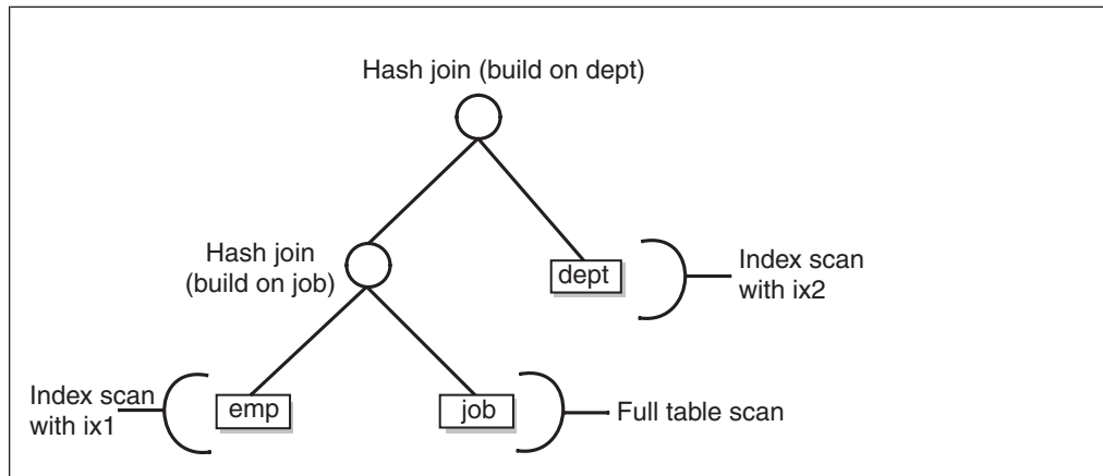
Figure 11-3. Possible query plan with directives
