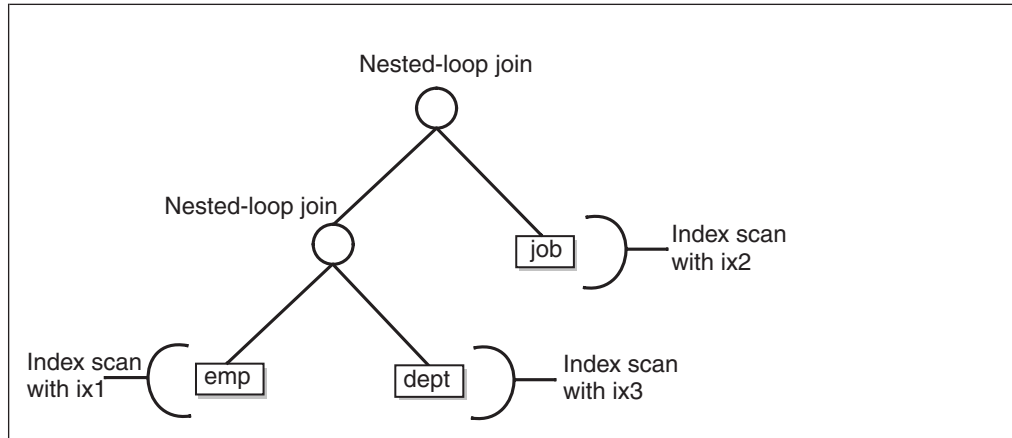
Figure 11-2. Possible query plan without directives
