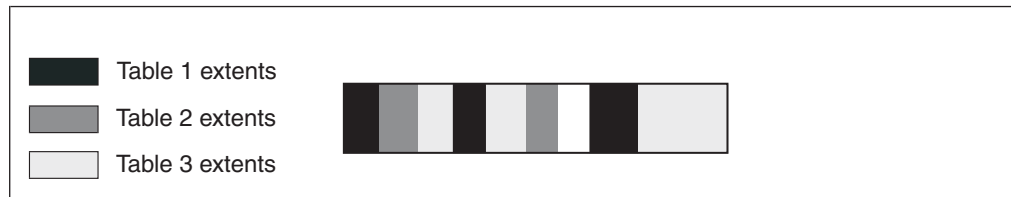
Figure 6-10. Interleaved table extents
