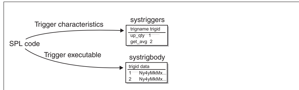
Figure 10-19. Trigger information stored in system catalog tables
