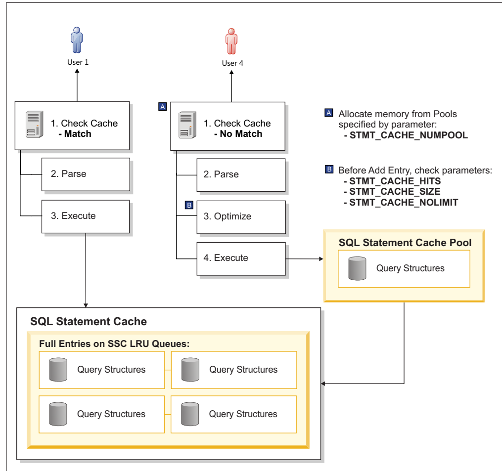
Figure 4-4. Configuration parameters that affect the SQL statement cache
