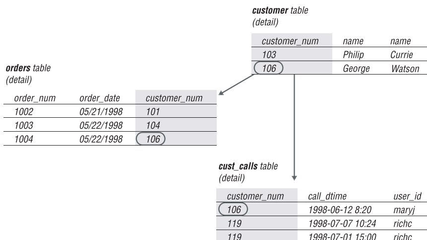
Figure 6-4. Referential integrity in the demonstration database
