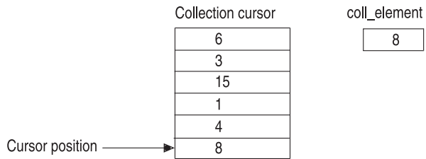
Figure 5-7. Collection cursor after fetch absolute 6
